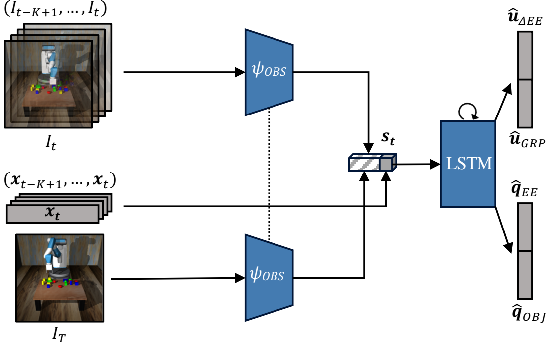
Figure 5.1: Model architecture of GEECO- \mathcal{R} . The same encoder \psi_{OBS} is used for RGB observations I_t and the target frame I_T . For each observed image I_t , the residual feature w.r.t. to the target image I_T is computed as \psi_{OBS}(I_T) - \psi_{OBS}(I_t) , indicated by the striped box in \mathbf{s}_t .
