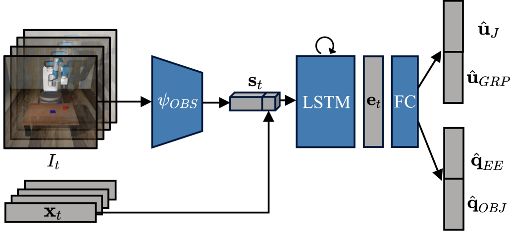
Figure 3.1: E2EVMC [42] model architecture. The current visual observation I_t is passed through a CNN \psi_{OBS} and concatenated with the proprioceptive feature \mathbf{x}_t to form the current state representation \mathbf{s}_t . This state representation \mathbf{s}_t is then fed into an LSTM to obtain the current embedding \mathbf{e}_t . The LSTM embedding \mathbf{e}_t is finally passed through a fully connected layer and decoded into action commands \hat{\mathbf{u}}_J and \hat{\mathbf{u}}_{GRP} , as well as auxiliary position predictions \hat{\mathbf{q}}_{EE} and \hat{\mathbf{q}}_{OBJ} .
