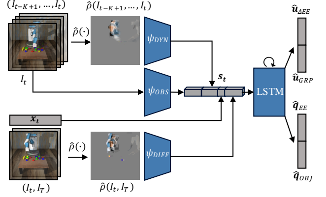
Fig. 3: Network architecture of GEECO-F. The observation buffer (I_{t-K+1}, \dots, I_T) is compressed into a dynamic image via \hat{\rho}(\cdot) and passed through \psi_{DYN} . The current difference to the target frame I_T is also computed via \hat{\rho}(\cdot) and passed through \psi_{DIFF} . Lastly, the current observation I_t is encoded via \psi_{OBS} . All CNNs compute spatial feature maps which are concatenated to the tiled proprioceptive feature \mathbf{x}_t . The LSTM's output is decoded into command actions \hat{u}_{\Delta EE} and \hat{u}_{GRP} as well as auxiliary pose predictions \hat{q}_{EE} and \hat{q}_{OBJ} .
