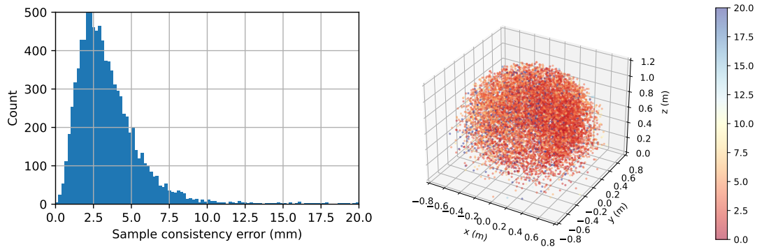
Figure 6.2: Analysis on latent space representation. Left: histogram of sample consistency errors from 10,000 prior samples. Right: 3d scatter of sample consistency errors at different end-effector positions.
