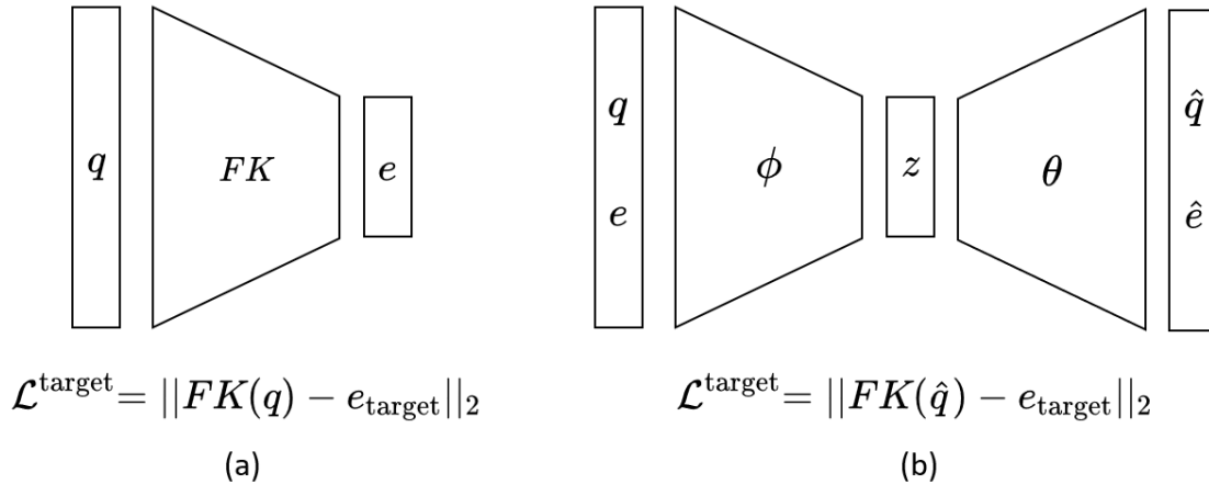
Figure 6.1: Alternative model designs. (a) Use the forward kinematics relationship and perform optimisation directly on the joint configuration \mathbf{q} . (b) Learn a latent representation \mathbf{z} as previously done, but formulate the target loss function using the reconstructed joint configuration \hat{\mathbf{q}} instead of the reconstructed end-effector position \hat{\mathbf{e}} .
