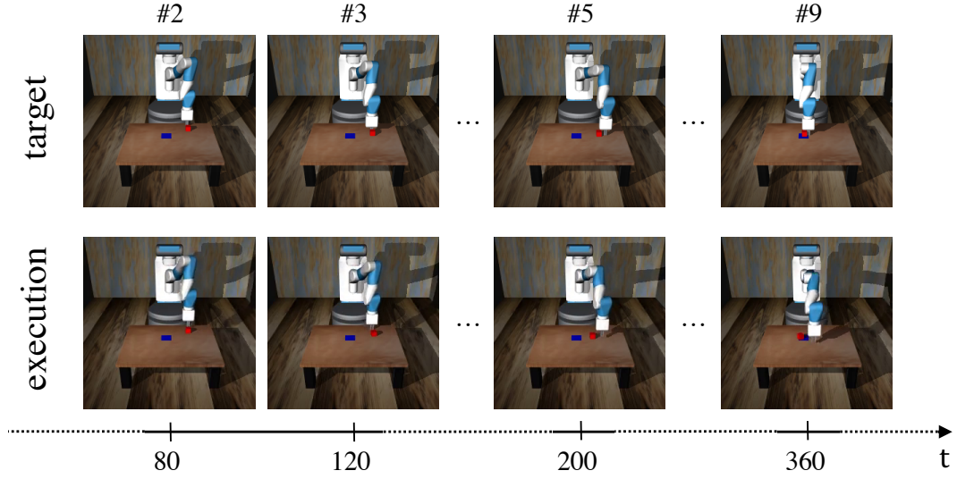
Figure 5.3: An execution of VFS with the ‘ground truth bottleneck’ scheme. The top row depicts intermediate target images from an expert demonstration. The bottom row shows the corresponding state of execution via VFS at time step t .
