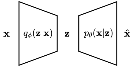
Figure 3.3: VAE model architecture: an input \mathbf{x} is passed through the encoder q_\phi(\mathbf{z}|\mathbf{x}) and embedded to a latent representation \mathbf{z} . This representation is then passed through the decoder p_\theta(\mathbf{x}|\mathbf{z}) and reconstructed as \hat{\mathbf{x}} .
