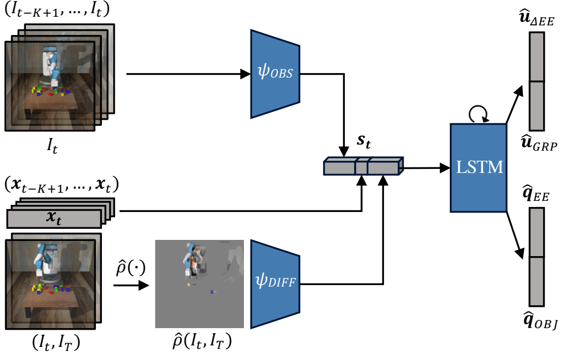
Figure 5.2: Model architecture of GEECO-D. For each image I_t in the observation buffer, the dynamic difference to the target image I_T is computed using \hat{\rho}(\cdot) . The difference image \hat{\rho}(I_t, I_T) is encoded with \psi_{DIFF} before being concatenated to s_t .
